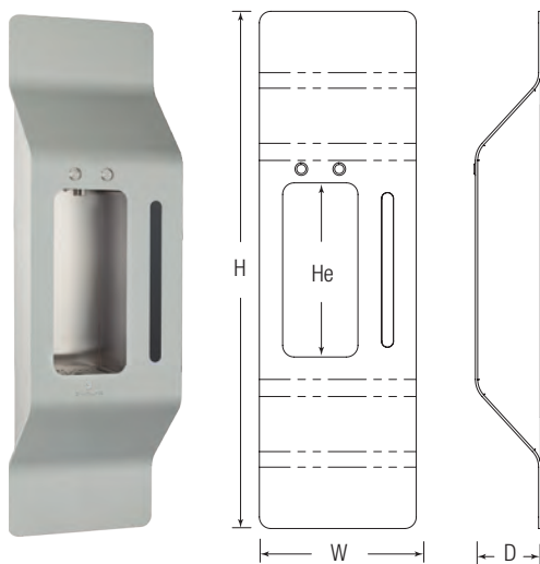
WALL - WALL "TOUCH FREE"
